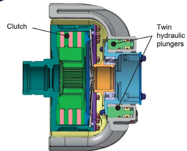
Fig. 5 Appearance of Direct Push Clutch (DPC)
