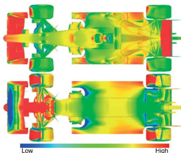
Fig. 4 Surface static pressure
