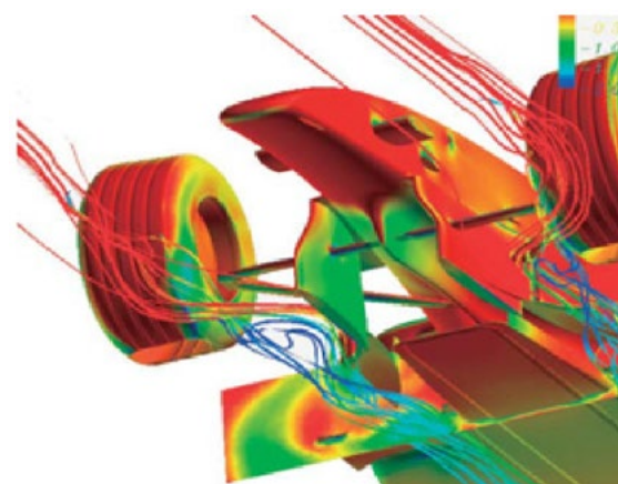
Fig. 18 ONF suction
