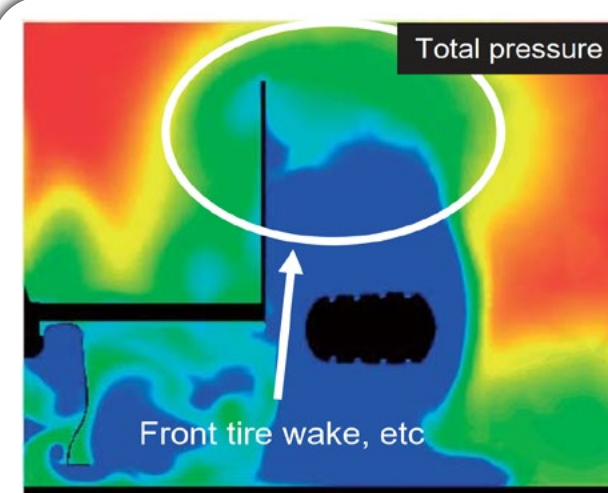
Fig. 38 Cp total around RW
