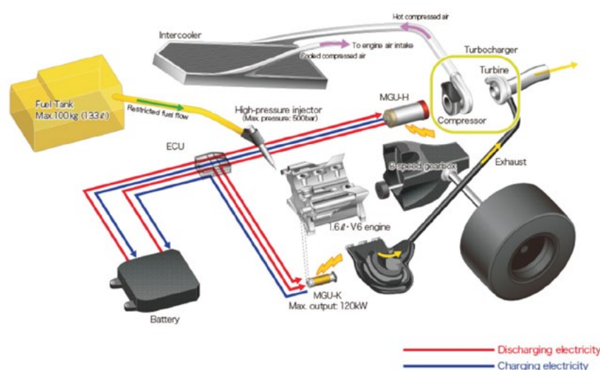
Fig. 6. Power Unit configuration and operation [20]
