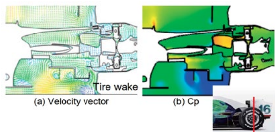
Fig. 32 Flow around diffuser
