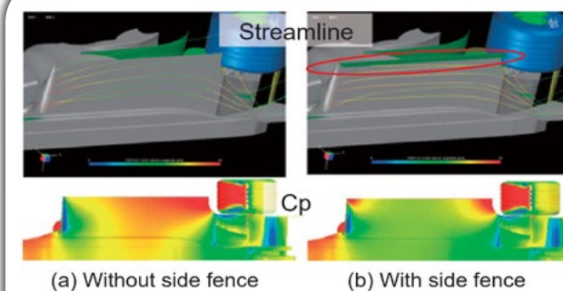
Fig. 24 Floor seal effect
