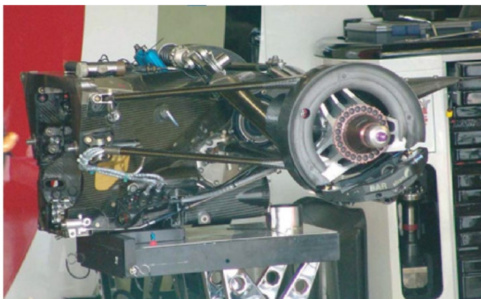
Fig. 1 Appearance of F1 gearbox
