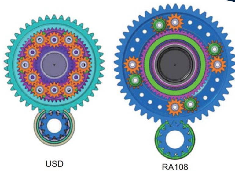
Fig. 6 Comparison between USD and RA108
