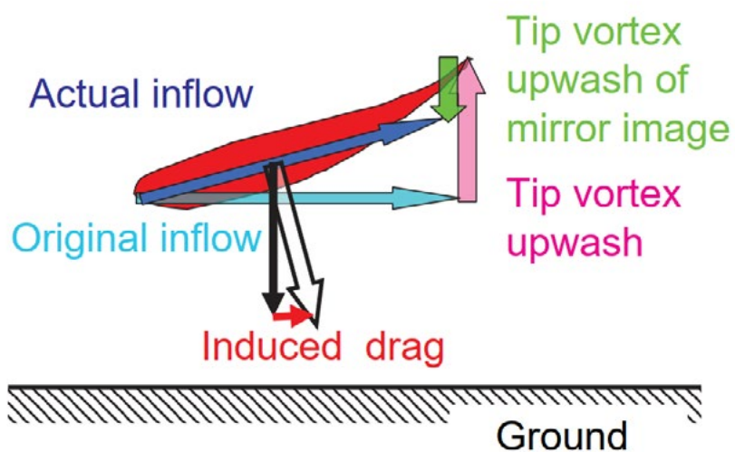
Fig. 2 3D ground effects
