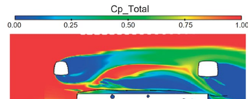
Fig. 7 Tire LE separation wake (CpT, Z=0 mm)
