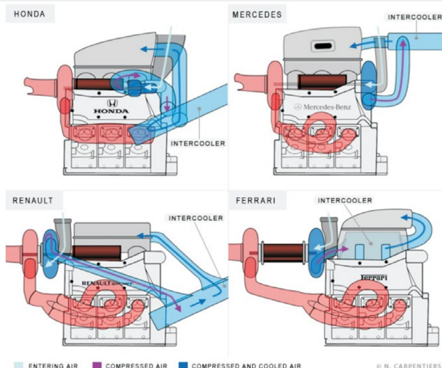
Fig. 7. Component layout of the Power Units [21]
