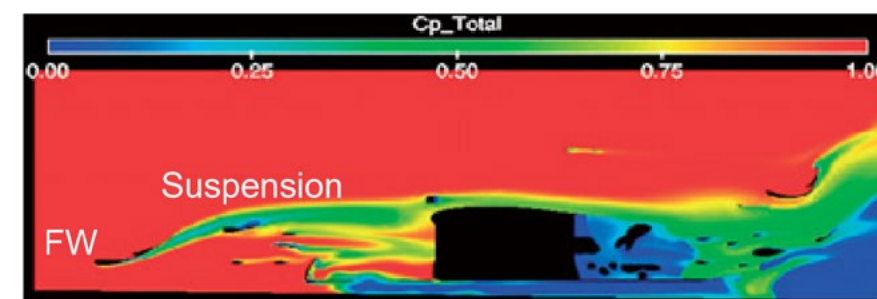
Fig. 6 Suspension stall (CpT, Y=300 mm)
