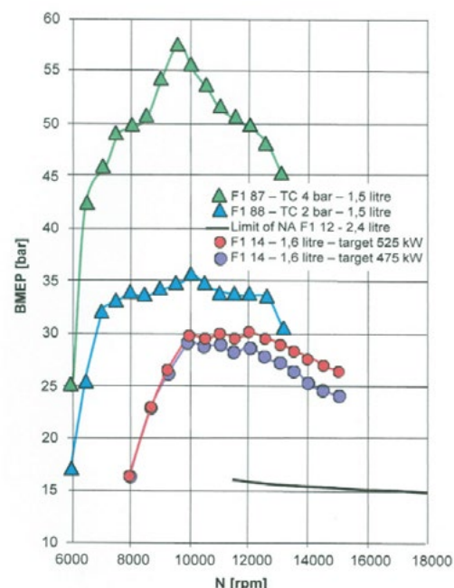
Fig. 1. Comparison of the BMEP of the turbocharged F1 engines of the mid - eighties with that of the modern F1 turbocharged engines [2, 13]
