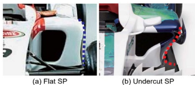
Fig. 23 Side pod variations
