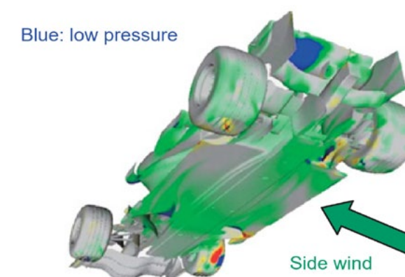
Fig. 11 Effect of bunny ears (delta Cp)
