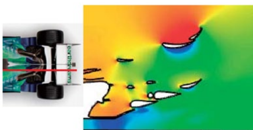
Fig. 34 Diffuser exit static pressure
