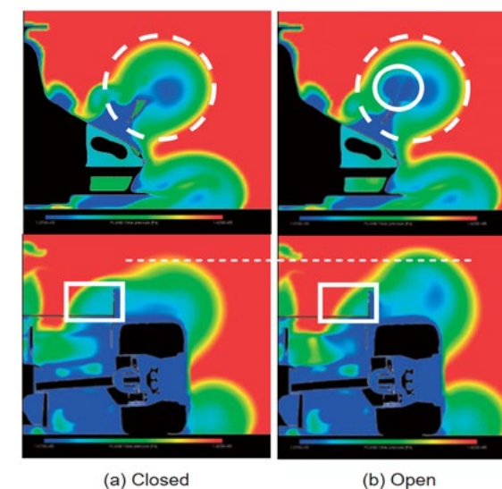
Fig. 29 Total pressure distribution in section around chimney trailing edge and RW leading edge
