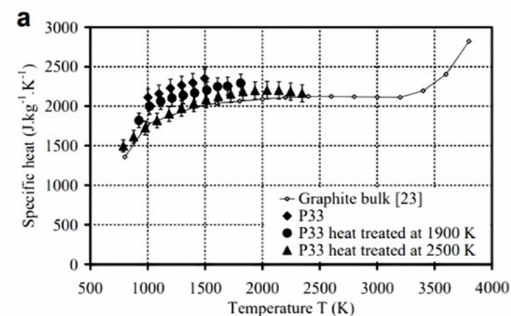
Figure 4: Specific heat to Temperature distribution of TC2
