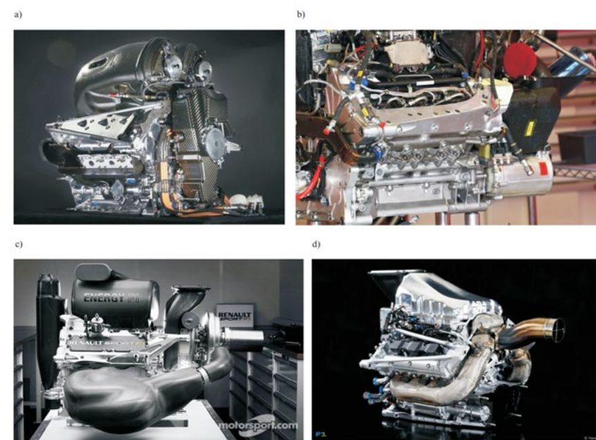
Fig. 5. F1 Power Units of the 2015 season: a) Mercedes AMG PU106B [16], b) Ferrari 059/4 [17], c) Renault RS25 Energy F1-2015 [18], d) Honda RA615H [19]
