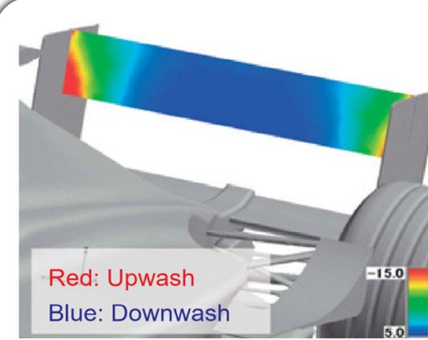
Fig. 37 Inflow angle for RW
