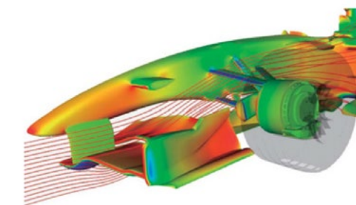
Fig. 9 FW upwash deflection by suspension arm
