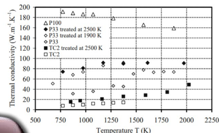
Figure 2: Thermal conductivity – temperature distributions of Carbon-Carbon polymers 5
