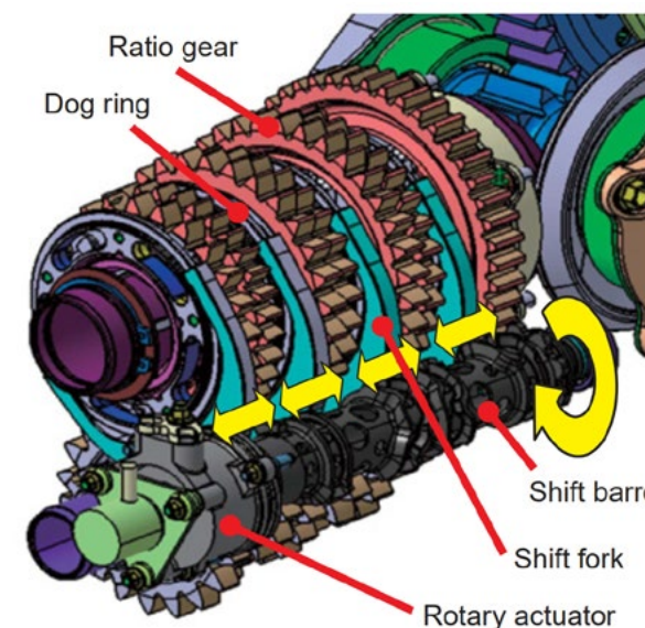
Fig. 3 Appearance of F1 gear-change system
