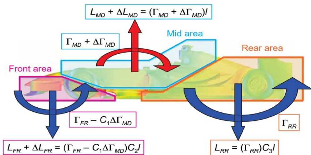
Fig. 3 Ideal chassis circulation
