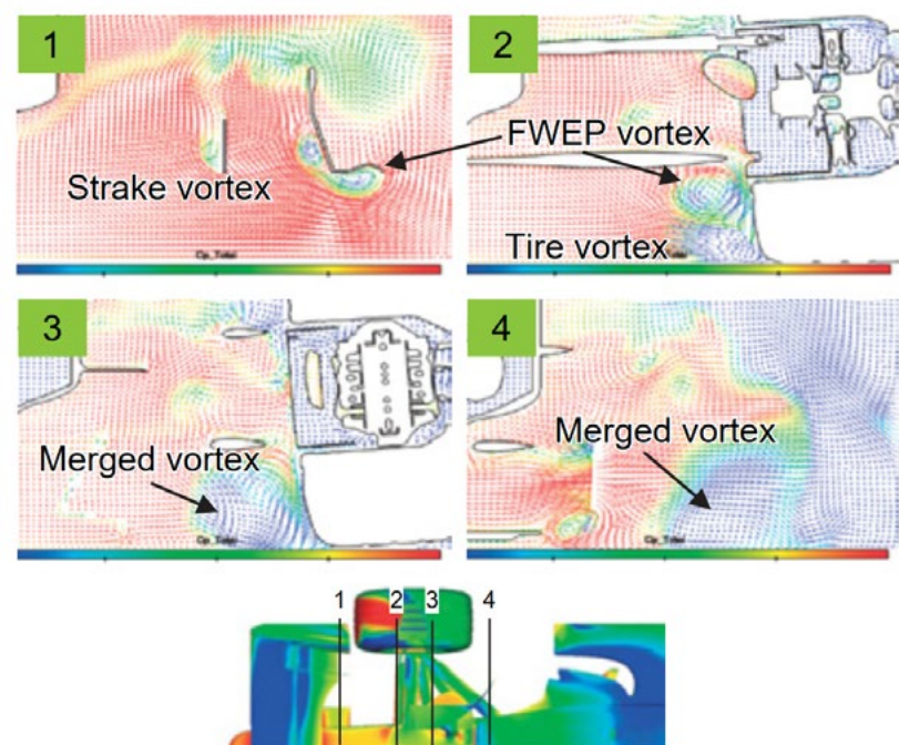
Fig. 8 FWEP and tire vortices (CpT, velocity vector)
