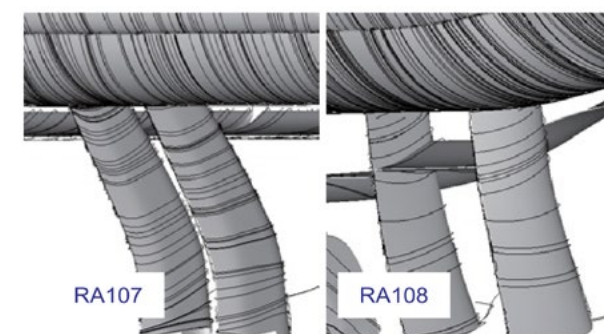
Fig. 42 Boundary layer shear direction on pillars
