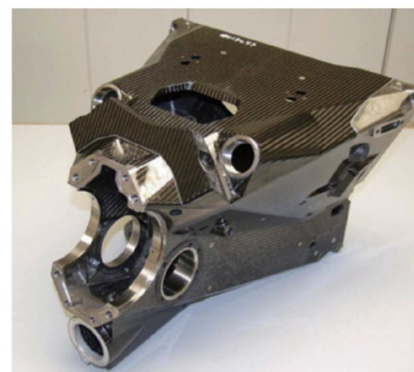
Fig. 4 Appearance of CFRP gearbox casing
